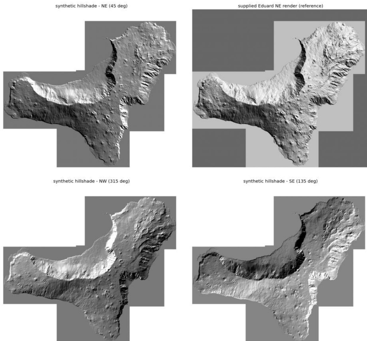
Figure 6: Synthetic hillshade on El Hierro from the steerable G_1 filters. Top row: synthetic NE ( 45^\circ , left) next to the supplied Eduard NE render (right; correlation 0.81). Bottom row: the same basis re-steered to NW ( 315^\circ ) and SE ( 135^\circ ), showing the illumination rotating coherently.
