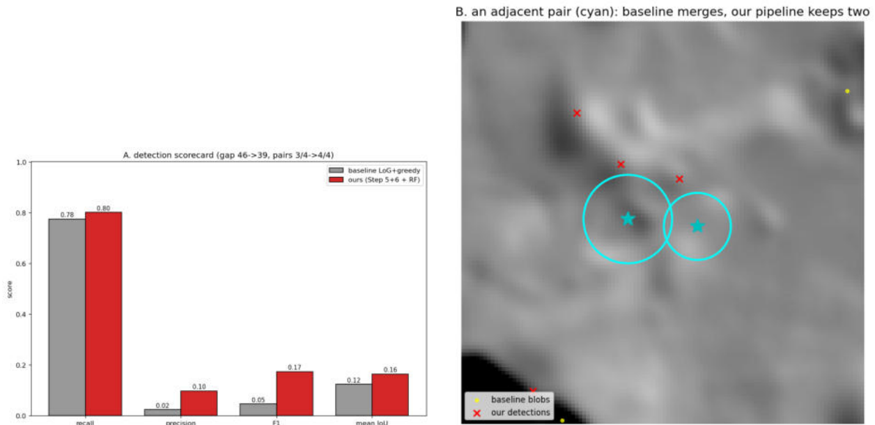
Figure 13: Step 8 on El Hierro. A : detection scorecard — the pipeline (red) beats the LoG + greedy baseline (grey) on recall, precision, F1 and IoU. B : a touching pair (cyan): the baseline blobs (yellow) collapse onto one cone, while our detections (red crosses) keep one on each.
