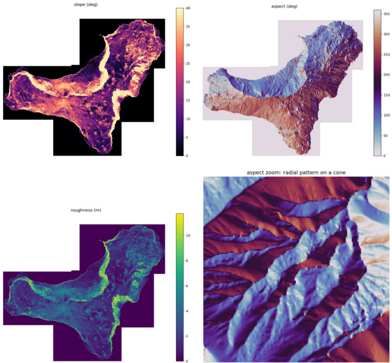
Figure 5: Morphometric channels derived from the El Hierro DEM: slope (top-left), aspect (top-right) and roughness (bottom-left), plus a zoom of the aspect (bottom-right) showing the radial pattern around a single cone.
