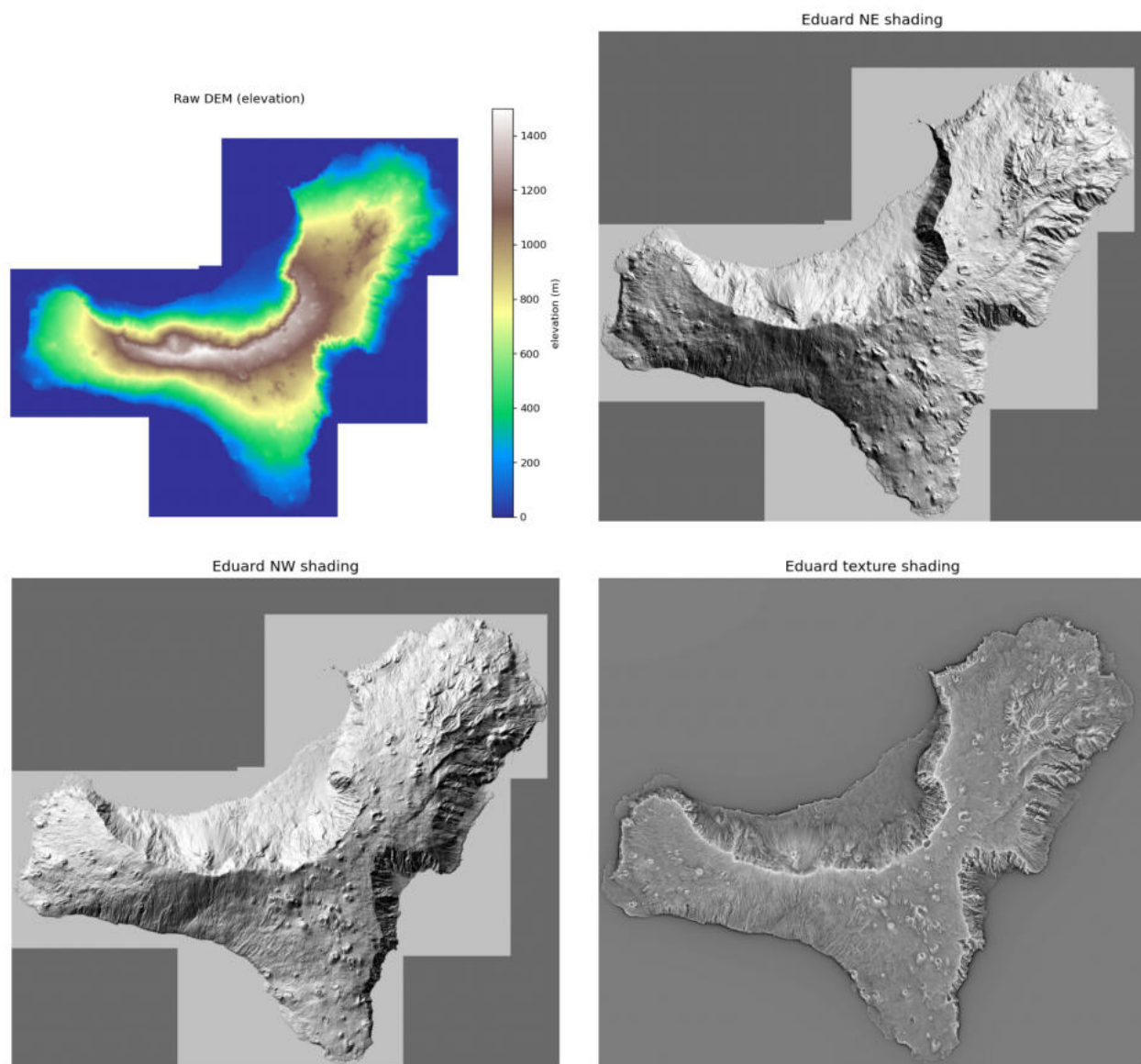
Figure 1: El Hierro: the raw DEM (top-left, colour bar in metres) is visually flat, while the Eduard renderings (NE and NW shading, top-right and bottom-left; texture shading, bottom-right) reveal the conical landforms.
